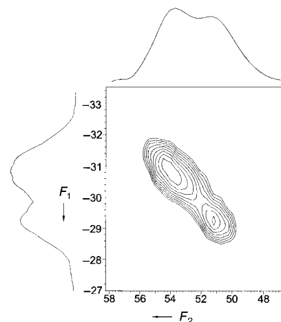
Figure 2. 2D ^{27}\text{Al} 3Q MAS NMR spectrum of an as-made ZSM-5 zeolite with Si/Al = 79 (1.2 Al atoms per unit cell). Two-peak maxima of tetrahedral Al atoms are clearly visible. The corresponding ^{27}\text{Al} MAS NMR spectrum is given at the top of the 3Q MAS NMR plot.
