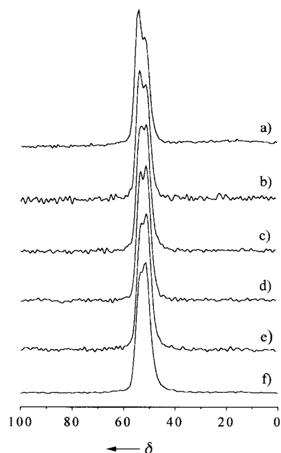
Figure 1. ^{27}\text{Al} MAS NMR spectra of as-made ZSM-5 zeolites with different Si/Al ratios: a) 250, b) 136, c) 79, d) 47, e) 27, and f) 14.
